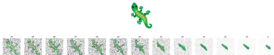
Figure 5.1: Denoising with Local Perception. The top image shows the target pattern used for training. The bottom row displays snapshots from a reverse diffusion process, which begins from a heavily noised version of the target and incrementally removes noise over 100 time-steps. The model is constrained to observe only local pixel neighborhoods. Although the system converges to a stable and locally self-consistent output, it fails to reconstruct many global features of the original pattern. This illustrates how local perception alone is insufficient for accurate reconstruction without additional disambiguating signals.
