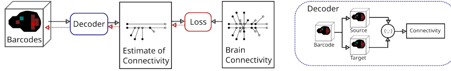
Figure 3.2: Architecture of the Static Model. ( Left ) The static model maps voxel-based latent variables (“barcodes”) through a decoder to produce an estimated voxel-to-voxel connectivity matrix. This estimate is then compared with empirical connectivity data, and the barcode parameters are optimized to minimize reconstruction error. ( Right ) The decoder architecture is shown. Each barcode is split into two disjoint sub-vectors, which are used to predict outgoing and incoming connections, respectively. Connectivity between any two voxels is estimated by taking the dot product between their corresponding sub-vectors. This figure introduces the general framework of mapping latent variables to connectivity patterns using a fixed decoder function—a setup that will be expanded in later chapters by incorporating developmental constraints.
