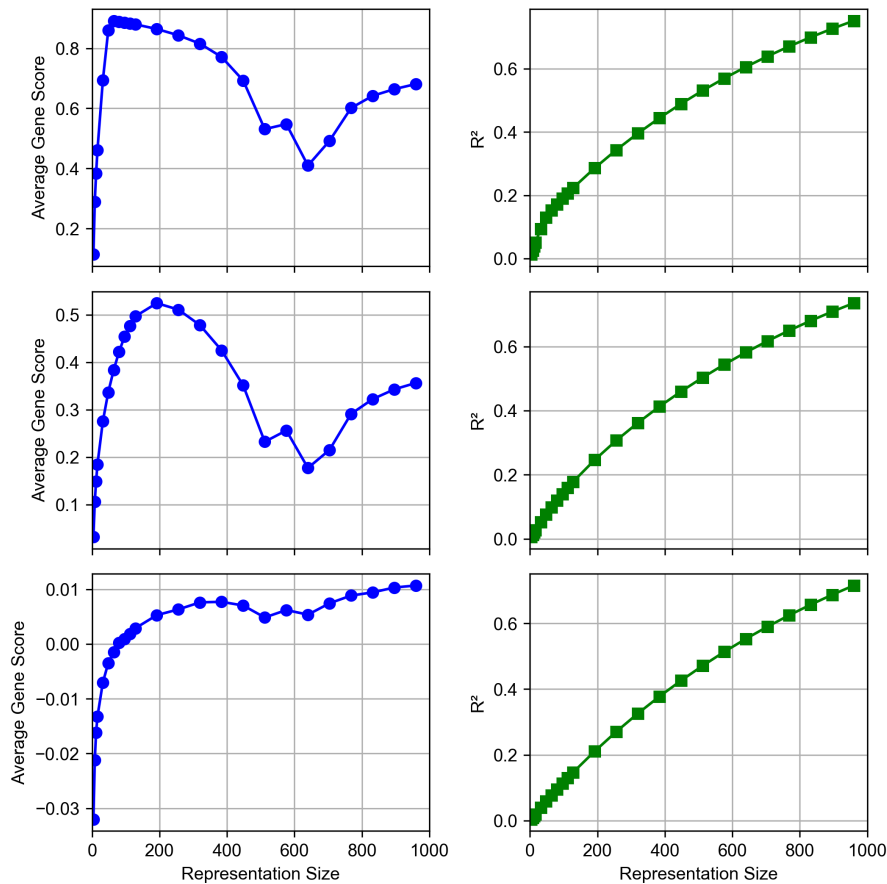
Figure 4.5: Model Complexity versus Data Complexity. In this figure, artificial data was constructed using “artificial barcodes,” random vectors with 50 ( top ), 200, ( middle ), or 10,000 ( bottom ) channels. These artificial codes formed the basis of an artificial connectivity matrix, which was then run through the same analysis pipeline used for the brain connectivity, resulting in gene scores ( left ) and R^2 ( right ) metrics. The figure indicates that the gene scores do pick up on the underlying complexity of the generated data for these artificially constructed datasets.
