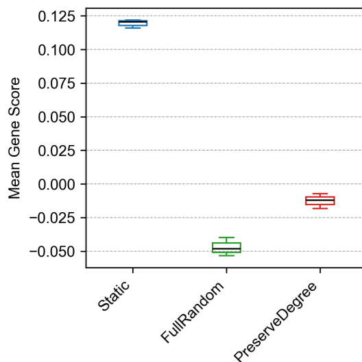
Figure 4.1: Genetic Predictivity of the Latent Variables. Gene scores are shown for a static model trained to predict either the true mouse brain connectivity or a set of randomized connectivity datasets. The distribution of gene scores for the true brain connectivity, compared to those for altered connectivity, indicates that structured wiring patterns drive the model’s predictions of genetic expression.
