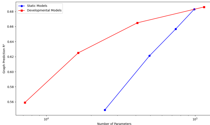
Figure 6.1: Complexity and Reconstruction Quality. The amount of the connectivity explained ( R^2 value) is plotted against the complexity of the model, for a selection of static and developmental models. The results indicate that small developmental models are particularly efficient representations of the connectivity.
