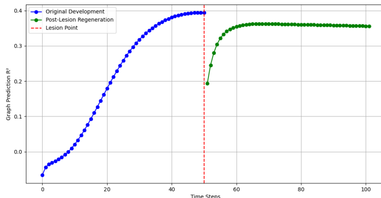
Figure 6.2: Repair After Injury. As the developmental model produces the initial pattern (blue curve), it incrementally builds up the predicted connectome, increasing the amount of the true brain network predicted ( R^2 ). Then, a lesion is applied to the system (red line). Despite being in a state it has never experienced during training, the developmental model is able to rebuild the ablated region (green curve) and partially recover the original predicted connectome. The plot illustrates the model’s capacity for self-directed structural repair.
