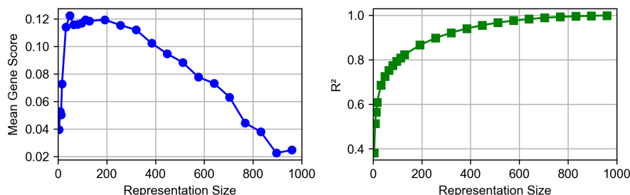
Figure 4.4: Tradeoff Between Model Complexity and Genetic Predictivity.
