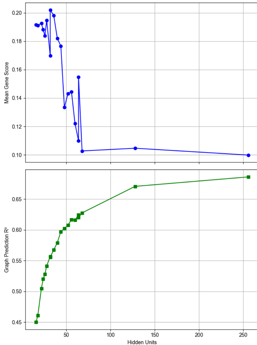
Figure 5.3: Tradeoff Between Model Complexity and Biological Predictivity. Gene scores (top) and connectivity reconstruction accuracy (bottom) are shown for developmental models at varying levels of complexity. As model complexity increases, reconstruction performance improves—but the ability to predict measured genetic expression declines. This tradeoff suggests that simpler models capture a structure more consistent with biological pattern formation.
