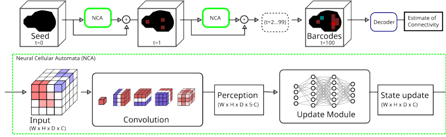
Figure 3.3: Architecture of the Developmental Model. ( Top ) The developmental model, implemented using an NCA block, process a sequence voxel-based states. It is initialized to a starting “seed” pattern at time t = 0 , which is repeatedly passed through the NCA to accumulate updates over multiple time steps. The final state, called the “barcodes,” is then passed through the decoder (described in the previous section) to produce a voxel-to-voxel estimate of brain connectivity. ( Bottom ) Internally, the NCA operates on a three-dimensional grid of vector-valued voxel states. At each time step, convolutional filters (identity, directional Sobel, and Laplace) are applied to extract a “perception vector” that encodes local spatial information. These vectors are processed by an update module—a small neural network—that computes the state updates of each voxel, the output of the NCA block. Thus the developmental architecture models connectivity as the outcome of a spatially local, iterative growth process, contrasting with the static model by incorporating temporal dynamics and neighborhood-based computation.
