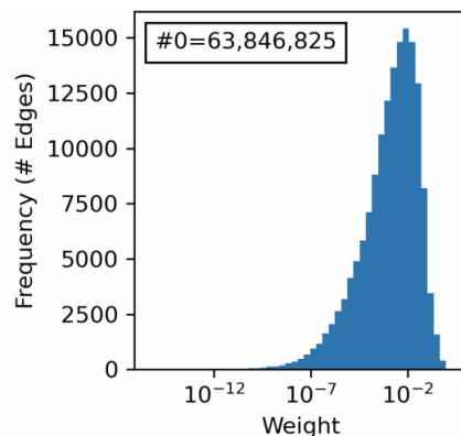
Figure 3.1: Brain Connection Weights. The distribution of connection weight values that is the raw output of the linear regression algorithm. These values span multiple orders of magnitude, which biases the resulting error gradient during learning so that the largest values take precedence. Post-processing to take the log of these values is therefore applied, allowing for all edges to contribute to the loss function on a similar scale.
